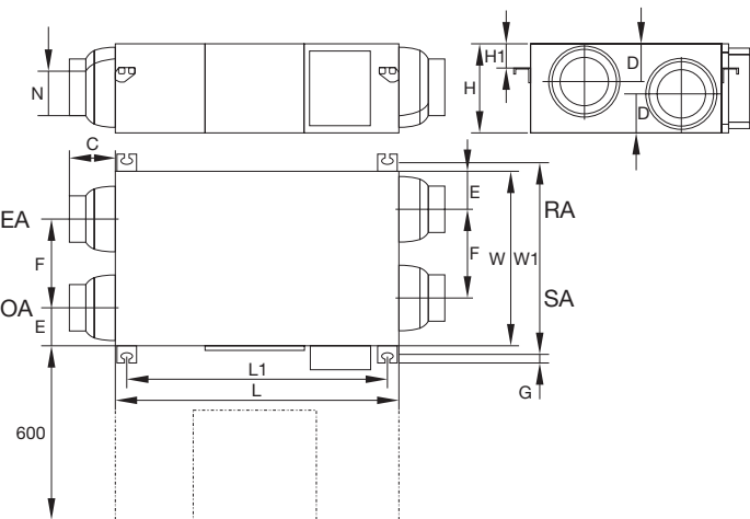
■ CHRU-TF 800 - CHRU-TF 1000
