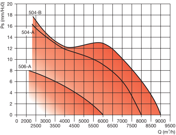
CAF / CAF ATEX 500
