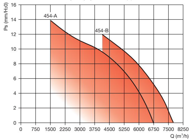
CAF / CAF ATEX 450
