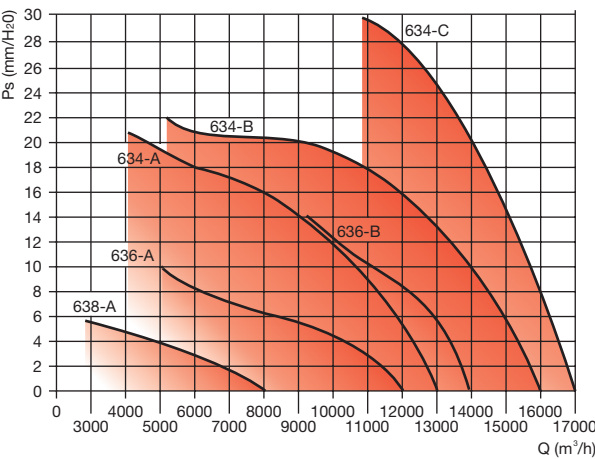
CAF / CAF ATEX 630
